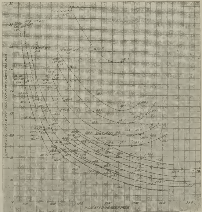
COMPARATIVE DIAGRAM OF INDICATED HORSEPOWER AND STEAM CONSUMPTION FOR L1S AND L10 LOCOMOTIVES.
